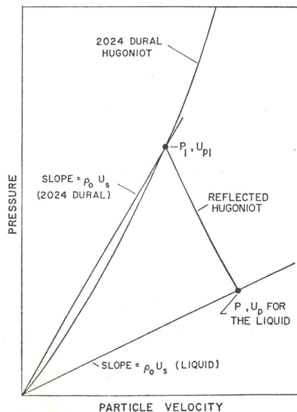
Fig. 1. Graphic representation of the impedance match method.
